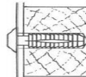
Rivet expands in solid furring strips, studs, substrates of brick block, concrete, drywall
