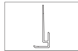
AP-34 Outside Corner for .150" Panel
