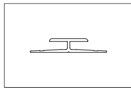
AP-30 Division Bar for .150" Panel
