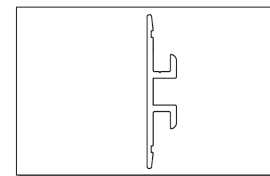
AP-103 Reveal for .150" Panel
