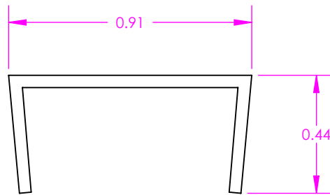
Left View
