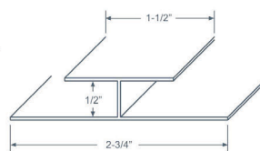
Division Bar
