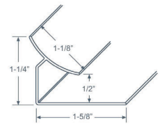
Inside Corner
