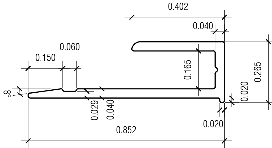
1 SIDE VIEW scale: NTS
